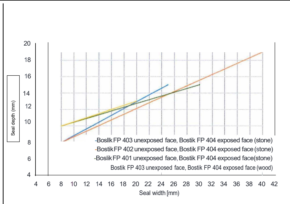
Graph 1: Minimum seal depth in relation to the seal width
